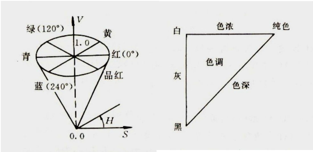
HSV
